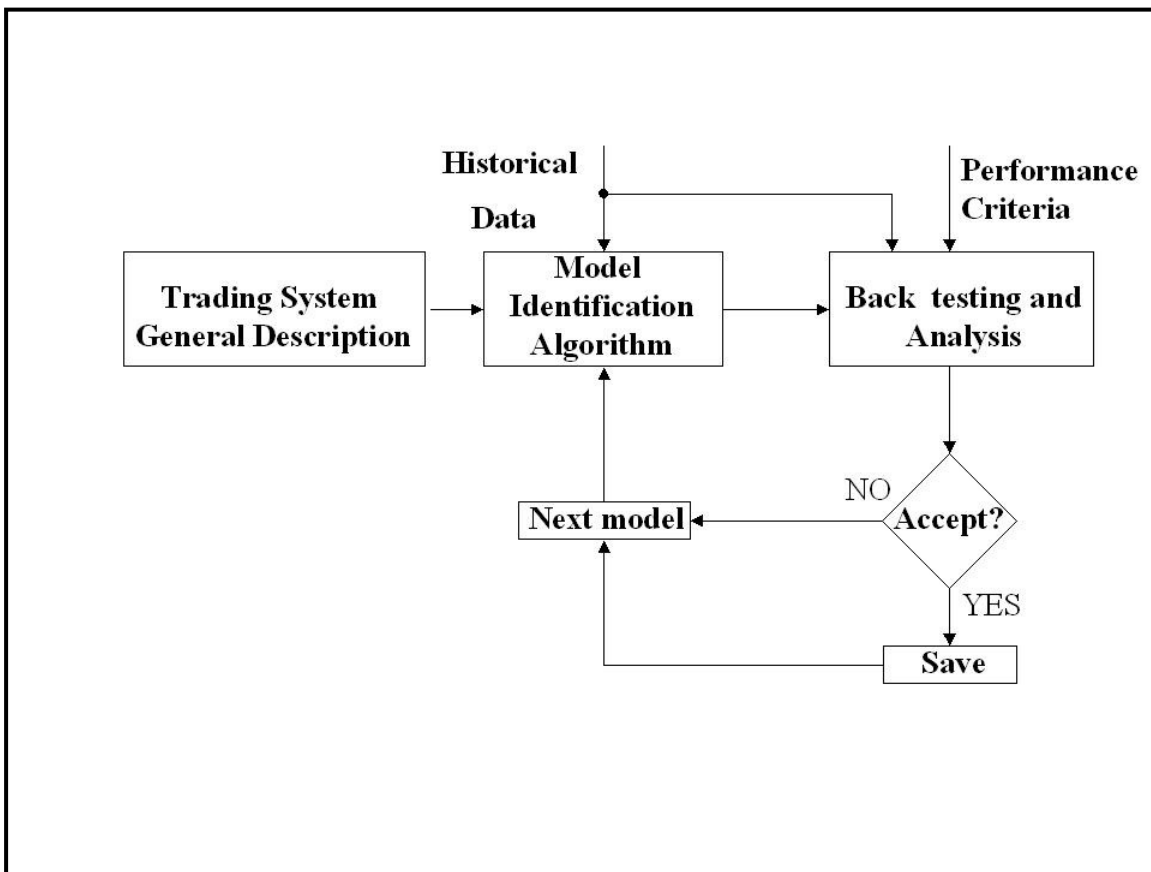
Figure 2. Development of trading systems using Synthesis
